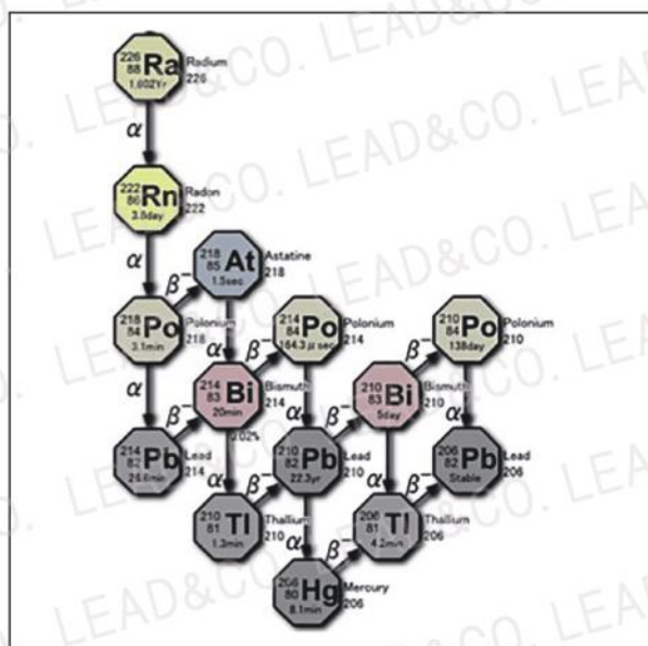
Figure 1. Radioactive decay chain of 222 Rn.
